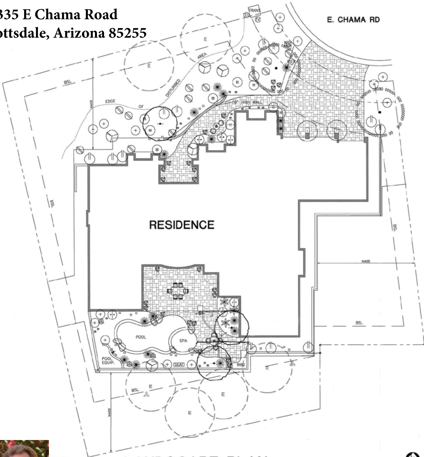
LANDSCAPE PLAN
